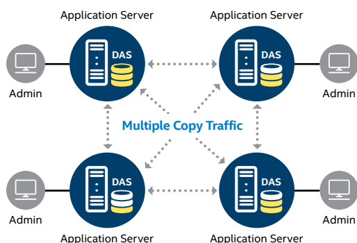
Figure 2. The DAS model (left) illustrates the drawbacks of conventional data center storage. In contrast, NVMe/TCP with ADQ technology and Lightbits LightOS allow for easy to deploy, modular, scalable, centrally managed storage over Ethernet connections.
