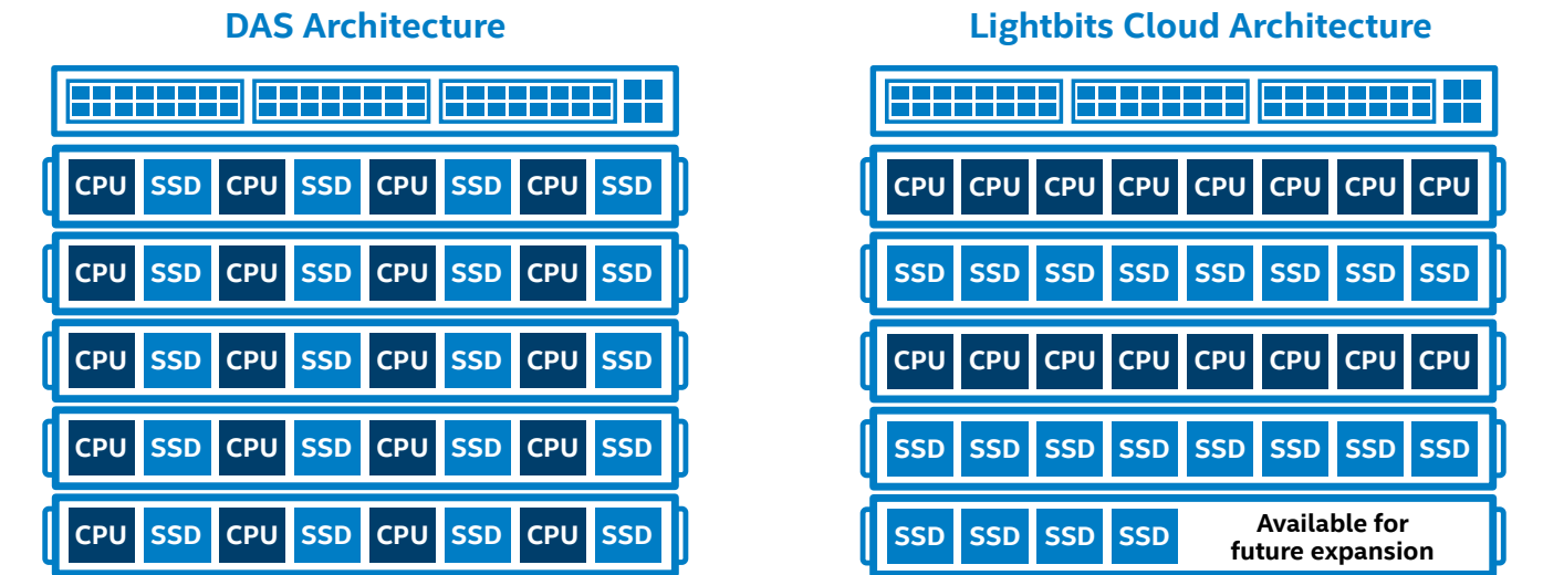
Figure 6. The “disaggregation” of storage through an NVMe/TCP and LightOS solution leads to a more efficient, scalable architecture in which compute and storage resources serve as flexible, modular blocks rather than inherently bound-together resources.
